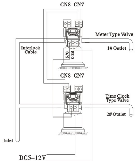
Figure 3-13 Series system
