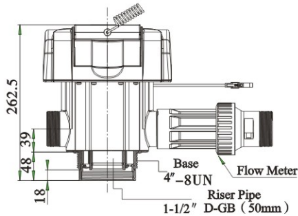
Structure Chart of F74B3 ( 63610B )
