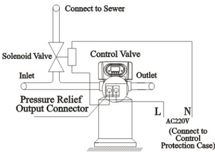
Figure 3-10 Wiring of Pressure Relief Output
