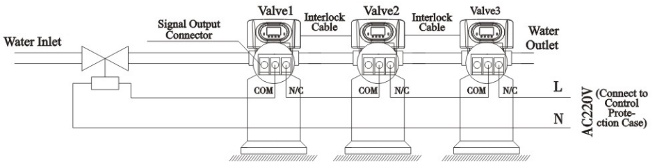
Figure 3-4 Wiring of Solenoid Valve in Inlet
