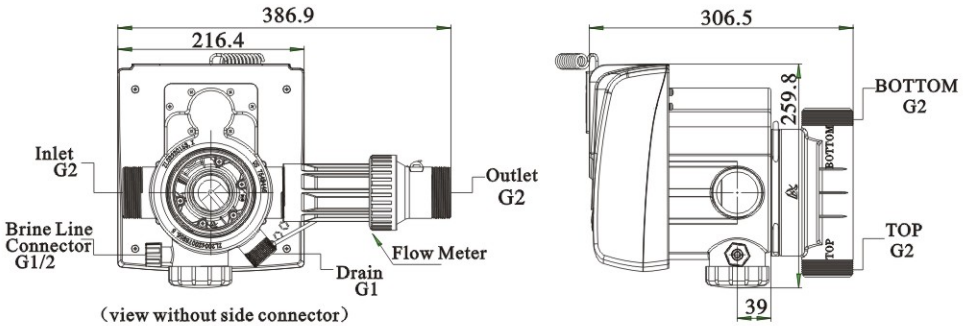
Structure Chart of N74A3 ( 63610 )
