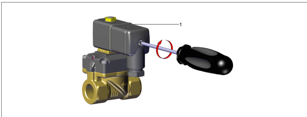
Fig. 6: Install the cable plug
